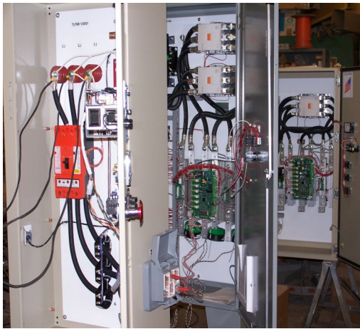
150HP Soft Start Pump Starter, 250HP Soft Start Fan Starter , and 1000V Distribution Panel
