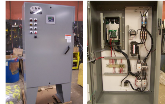
VFD for a belt conveyor at a cleaning facility
